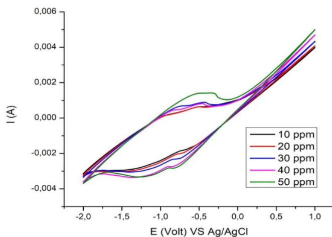
Fig. 5 Lead voltammogram with concentration of 10 – 50 ppm in citrate buffer solution pH 5 with 5 s deposition time and scan rate 100 mV/s
